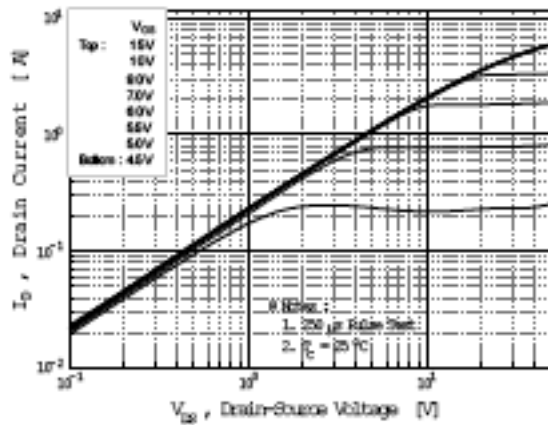
Fig 1. Output Characteristics
